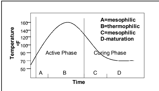
Figure 2. Temperature changes in an average compost pile.
